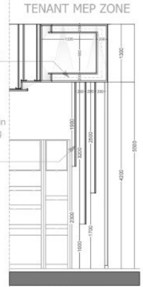
Section C-C
